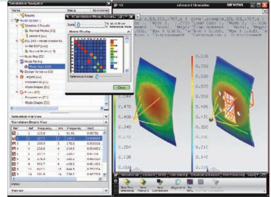
Side-by-side mode shapes test/analysis and MAC prior to model update.
